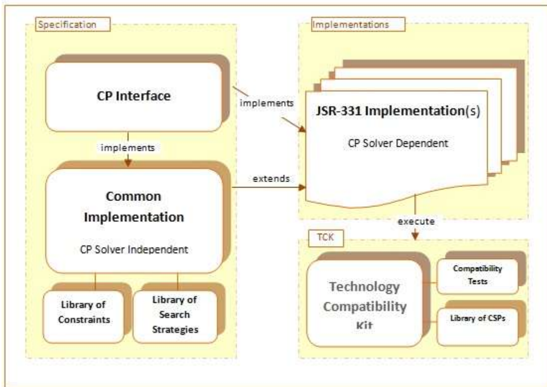
Figure 1. JSR-331 Architecture
